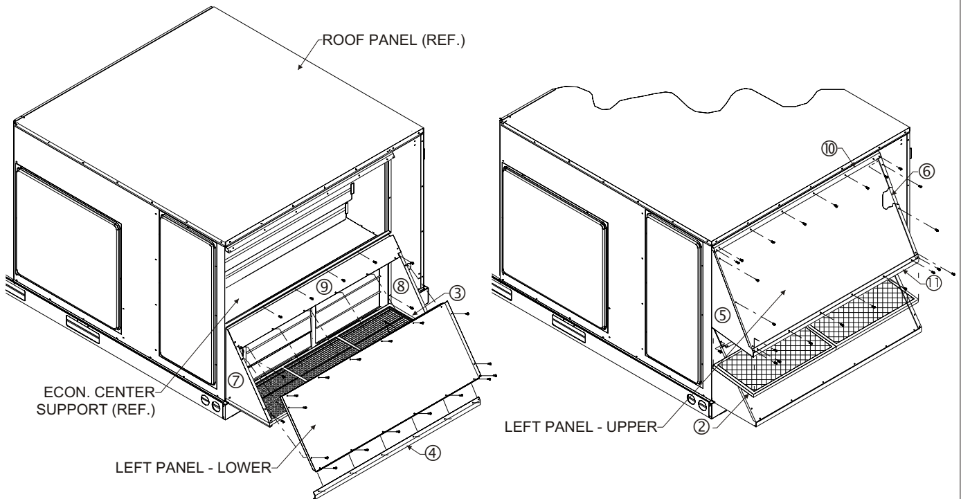
FIGURE 3 (-)XRD-01RJDCM3 Shown - (-)XRD-01RJDDM3 Similar (See Table 1 for identification of parts)
