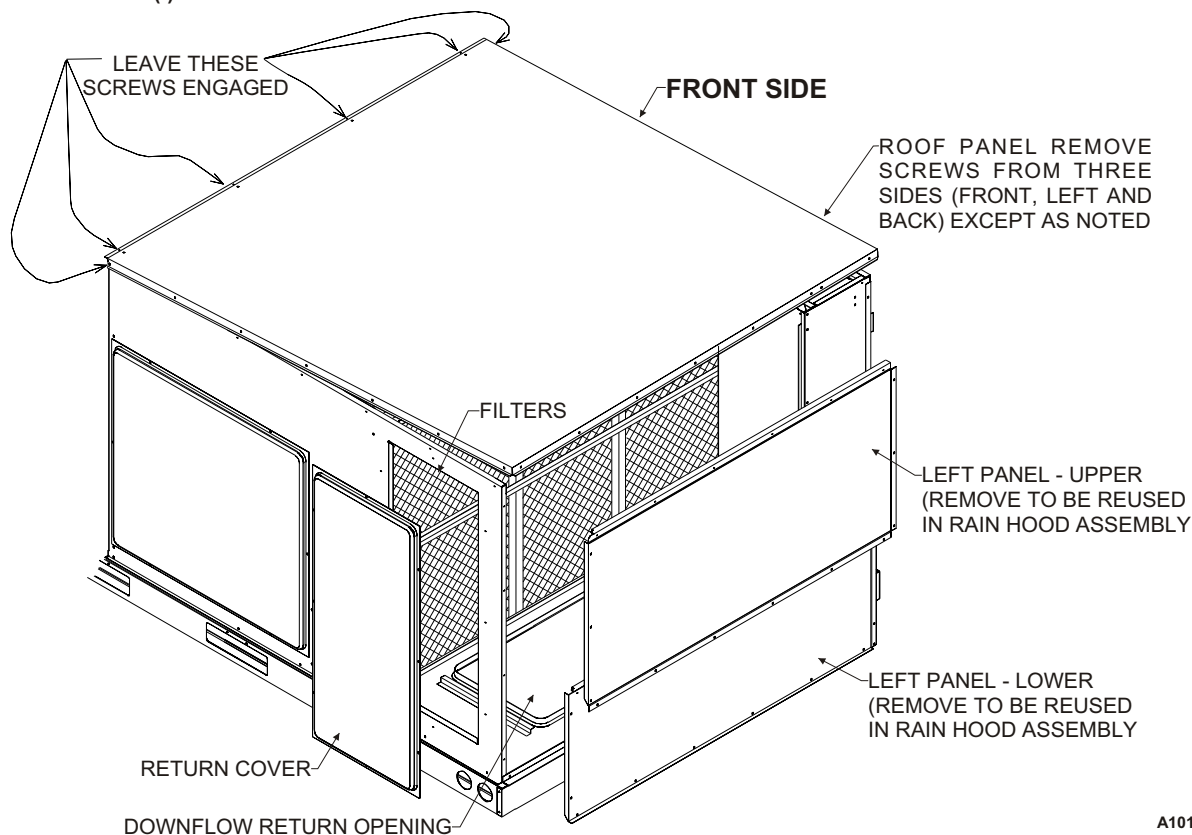
FIGURE 1 (-)XRD-01RJDCM3 Shown - (-)XRD-01RJDDM3 Similar
